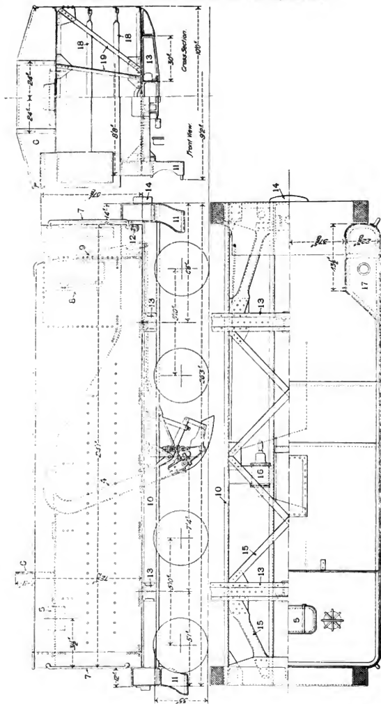
Figs. 4083-4085. General Arrangement of 5,000-Gallon Tender Tank for Atlantic (1-1-21) Locomotive, Pennsylvania Railroad.
